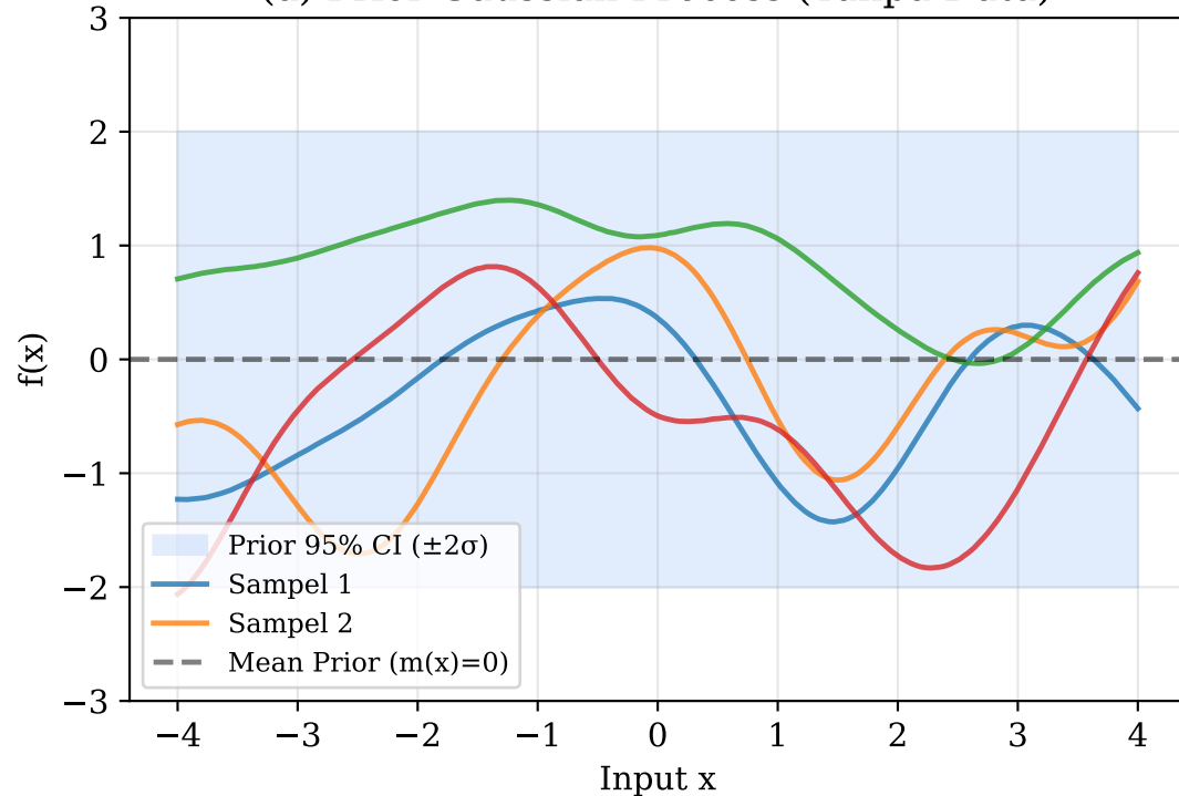
(a) Prior Gaussian Process (Tanpa Data)
